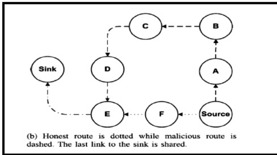
Fig. 3 - Carousal Attack Example
