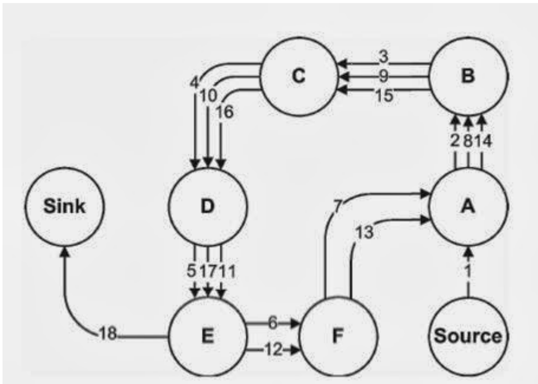
Fig. 4 - Example of Stretch Module Attack
